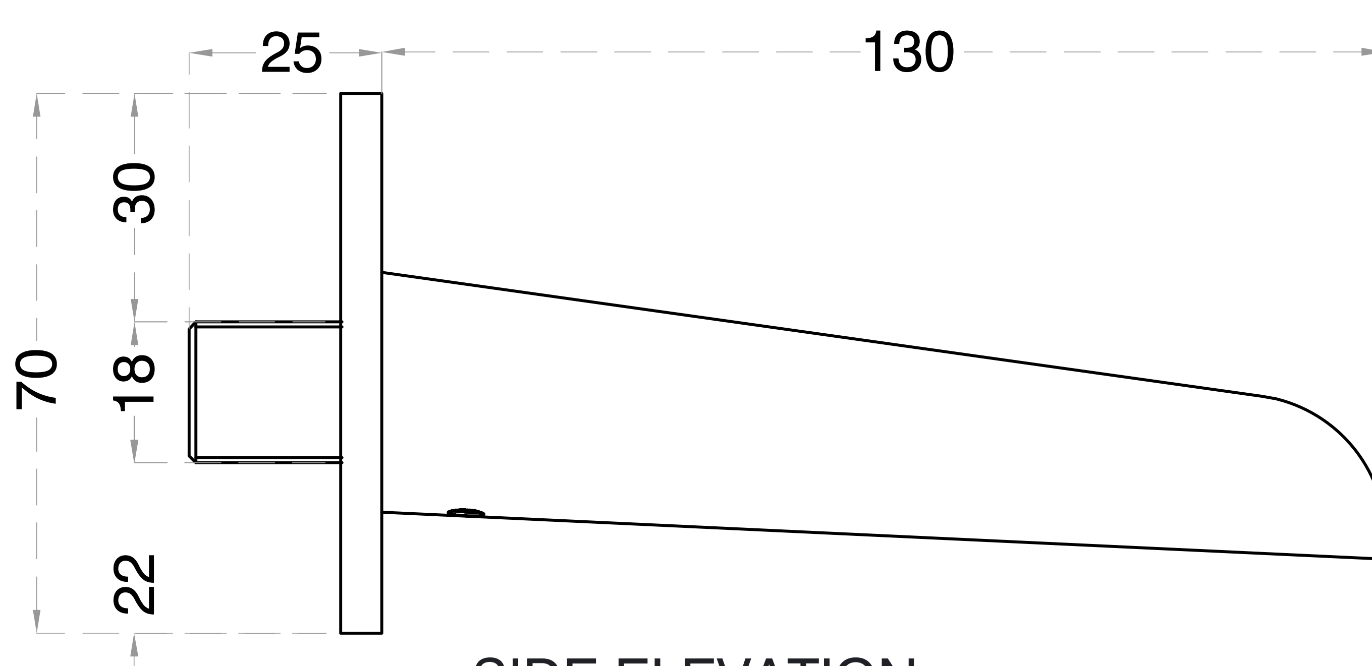
SIDE ELEVATION
